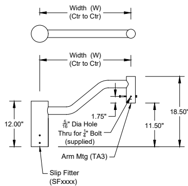
Single Arm (S1)
