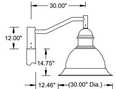
AT24 S1-1226 Single Arm, 12" H x 30" Ctr to Ctr with Washburn 30" (WAS-30/WASGG-30) & 5" Dia. Pole.
