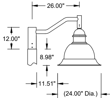
AT24 S1-1226 Single Arm, 12" H x 26" Ctr to Ctr with Washburn 24" (WAS-24/WASGG-24) on 5" Dia. Pole.
