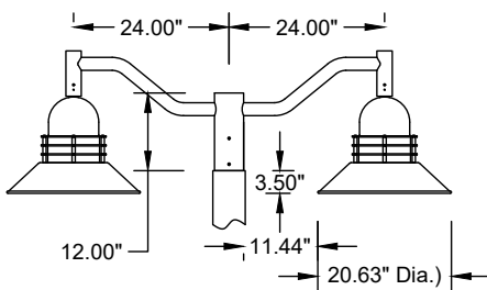
AT24 D180-2418 Double Arm, 12" H x 24" Ctr to Ctr with Premier 20" (PRM-20/PRMG-20) & 5" Dia. Pole.
