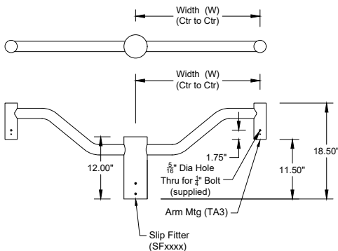
Double, Triple and Quad Arms (Dxx, Txx, Qxx) (Double Arm (D180) Shown for Clarity)
