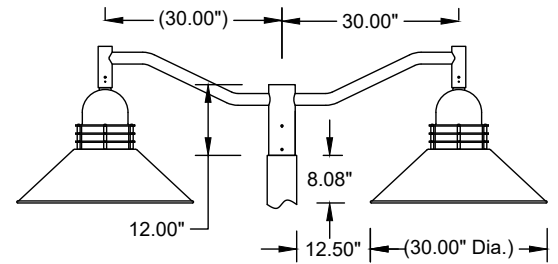
AT24 D180-1230 Single Arm, 12" H x 30" Ctr to Ctr with Premier 30" (PRM-30/PRMG-30)
