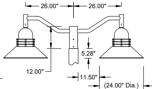
AT07 S1-4226 Double Arm, 12" H x 26" Ctr to Ctr with Premier 24" (PRM-20/PRMG-24)
