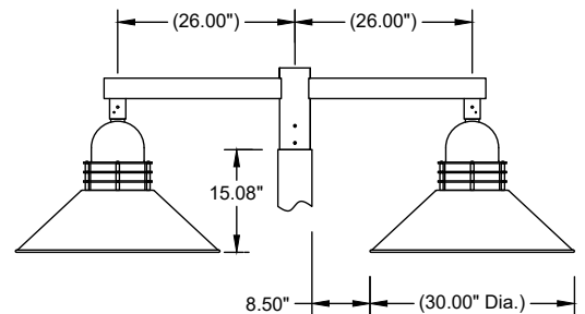
AT04 S1-1226 Single Arm, 12" H x 26" Ctr to Ctr with Premier 30" (PRM-30/PRMGG-30) on a 5" Dia. Pole.
