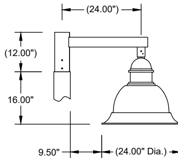
AT04 S1-1224 Single Arm, 12" H x 24" Ctr to Ctr with Washburn 24" (WAS-24/WASGG-24) on a 5" Dia. Pole.
