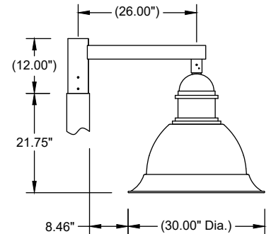
AT04 S1-1226 Single Arm, 12" H x 26" Ctr to Ctr with Washburn 30" (WAS-30/WASGG-30) on a 5" Dia. Pole.
