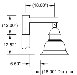
AT04 S1-1218 Single Arm, 12" H x 18" Ctr to Ctr with Washburn 18" (WAS-18/WASGG-18) on a 5" Dia. Pole.
