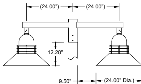
AT04 S1-1224 Single Arm, 12" H x 24" Ctr to Ctr with Premier 24" (PRM-24/PRMGG-24) on a 5" Dia. Pole.
