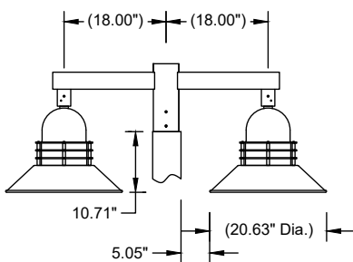
AT04 S1-1218 Single Arm, 12" H x 18" Ctr to Ctr with Premier 20" (PRM-20/PRMGG-20) on a 5" Dia. Pole.
