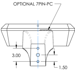
HOLES PATTERN
