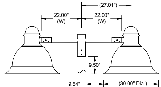
AT05 180-1222 Double Arm, 12" H x 22" Ctr to End with Washburn 30" (WAS-30/WASGG-30) on a 5" Dia. Pole.
