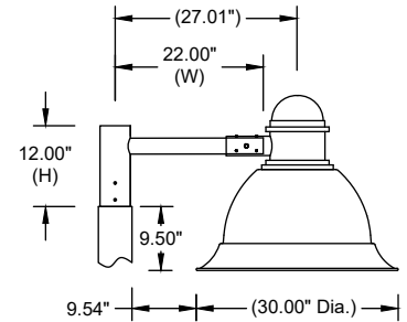
AT05 1222 Single Arm, 12" H x 22" Ctr to End with Washburn 30" (WAS-30/WASGG-30) on a 5" Dia. Pole.
