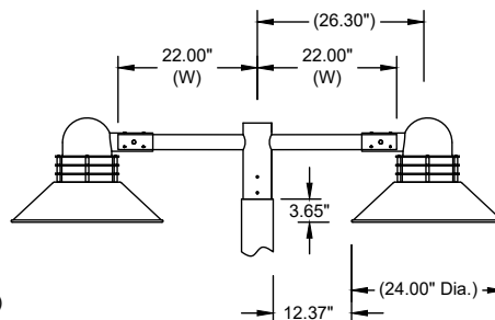
AT03 S1-1224 Single Arm, 12" H x 24" Ctr to Ctr with Premier 24" (PRM-20/PRMG-24) on a 5" Dia. Pole.
