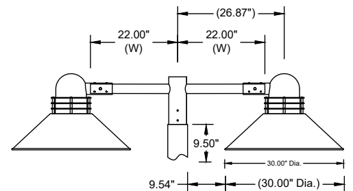
AT03 S1-1226 Single Arm, 12" H x 26" Ctr to Ctr with Premier 30" (PRM-20/PRMG-30) on a 5" Dia. Pole.
