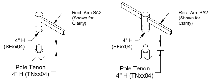
AT05 : Single Arm (S1) (SA2 - Rect. Arm Shown)
