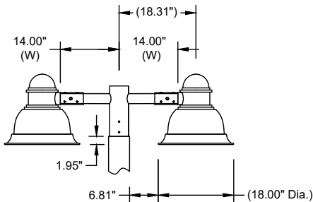
AT05 D18-1214 Double Arm, 12" H x 14" Ctr to End with Washburn 18" (WAS-18/WASGG-18) on a 5" Dia. Pole.
