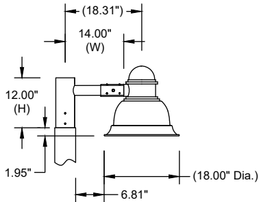
AT05 S1-1214 Single Arm, 12" H x 14" Ctr to End with Washburn 18" (WAS-18/WASGG-18) on a 5" Dia. Pole.
