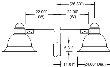
AT05 D180-1222 Double Arm, 12" H x 22" Ctr to End with Washburn 24" (WAS-24/WASGG-24) on a 5" Dia. Pole.
