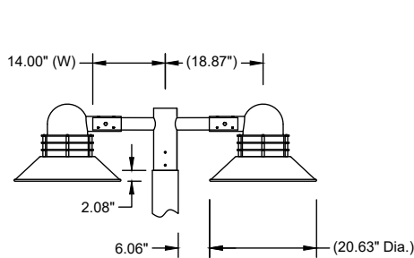
AT03 S1-1218 Single Arm, 12" H x 18" Ctr to Ctr with Premier 20" (PRM-20/PRMG-20) on a 5" Dia. Pole.
