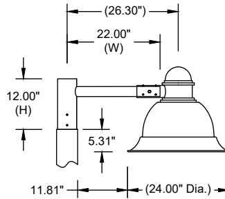
AT05 S1-1222 Single Arm, 12" H x 22" Ctr to End with Washburn 24" (WAS-24/WASGG-24) on a 5" Dia. Pole.
